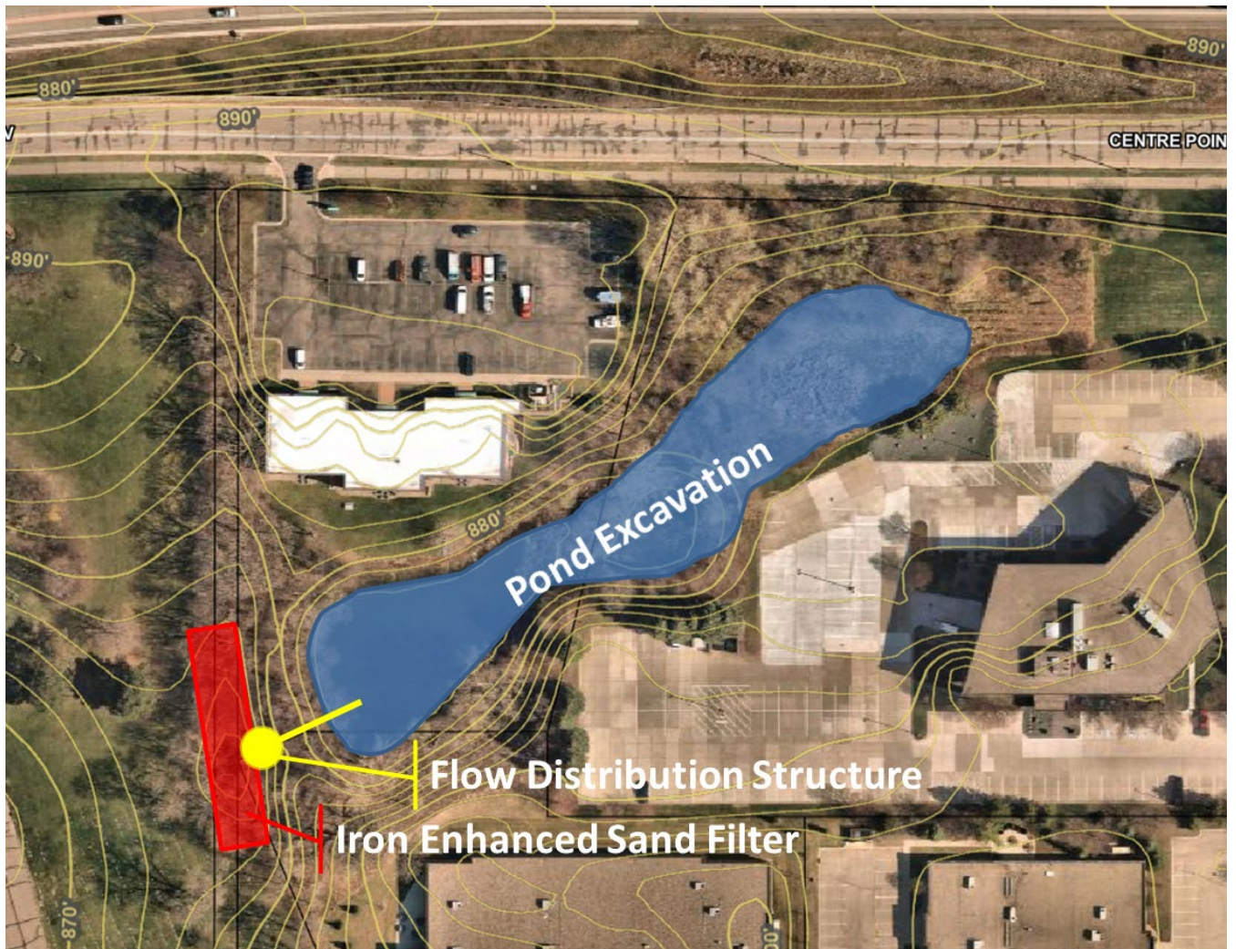
Figure 5-4 Conceptual Design of Stormwater Pond 2 Enhancements
